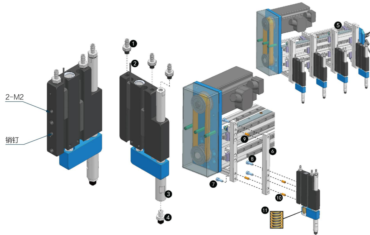
XD-0806-L-S 气缸配件和功能说明 Cylinder accessories and function description
